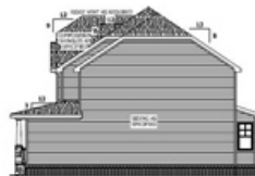
RIGHT SIDE ELEVATION SCALE 1/8" = 1'-0"
